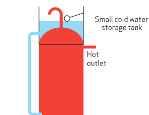
Figure 20: Fortic (type) tanks and pre-assembled units
