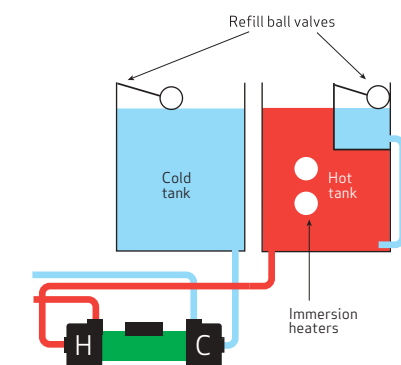
Figure 19: Elson (type) tanks
