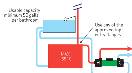
Figure 24: Horizontal cylinders
