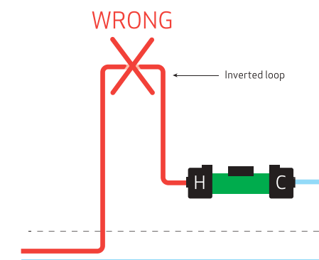
Figure 27: Inverted loops
