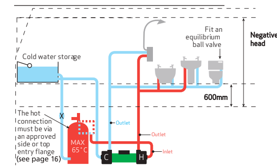
Figure 9: Negative head
